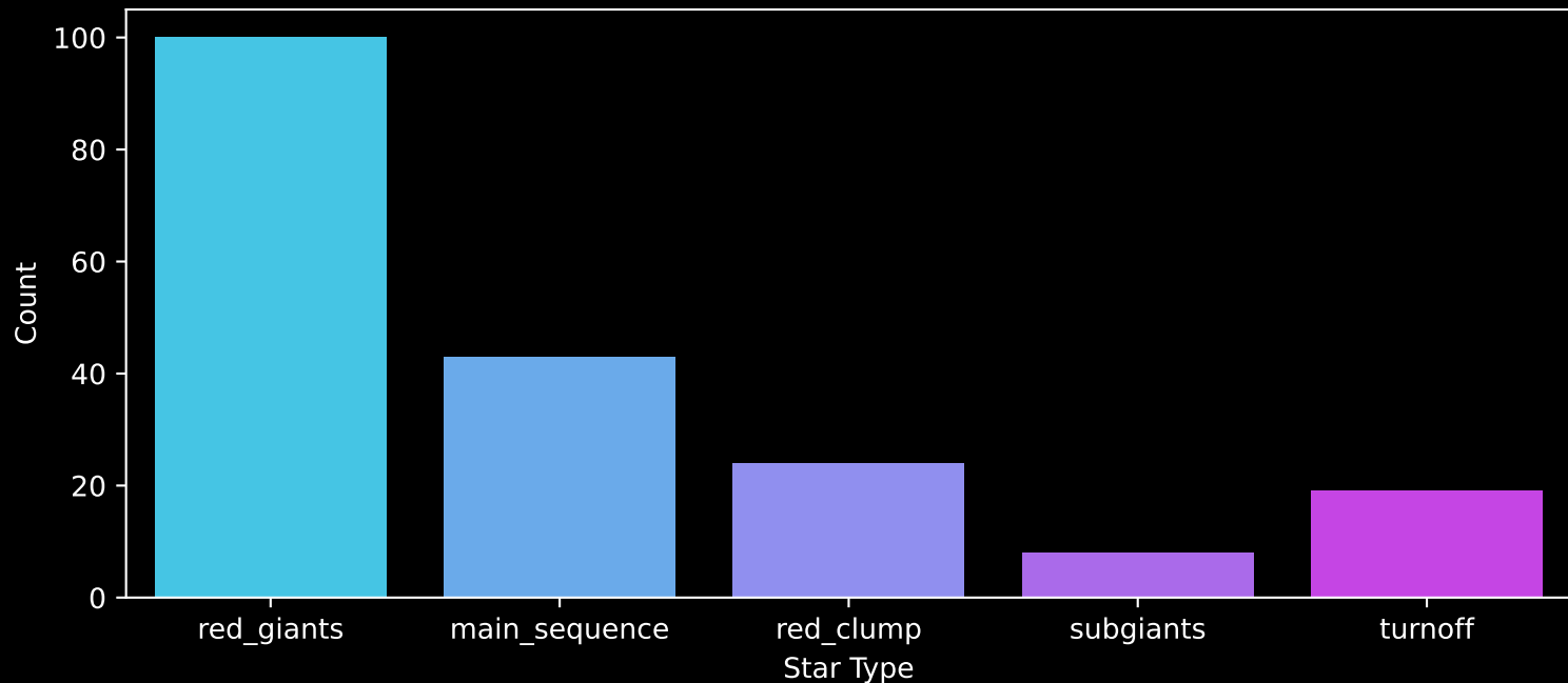
APOGEE DR17 Field: [210+16] Count plot of Star Type
