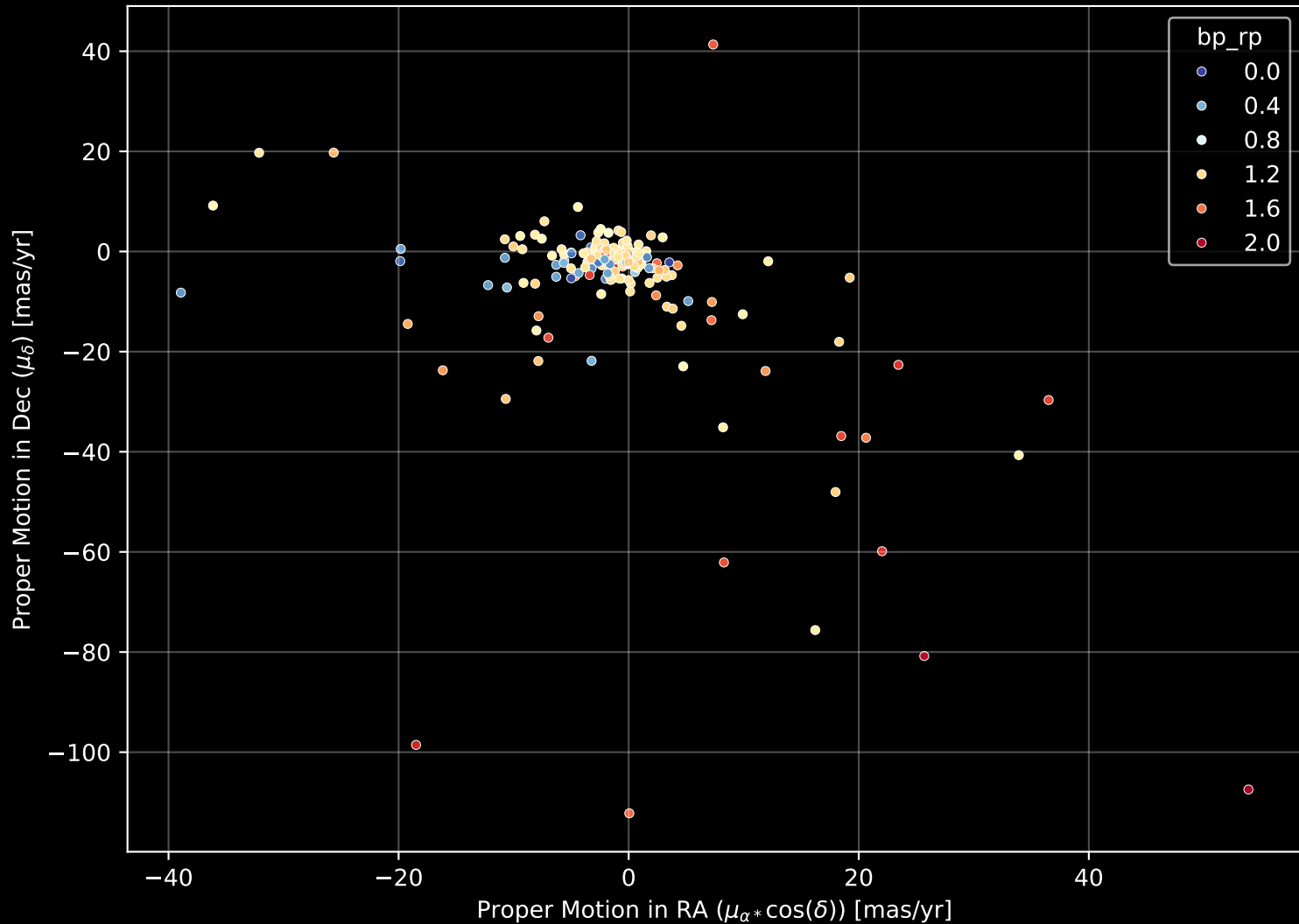
APOGEE DR17 Field: [210+16] Proper Motion Diagram (n= 194)
