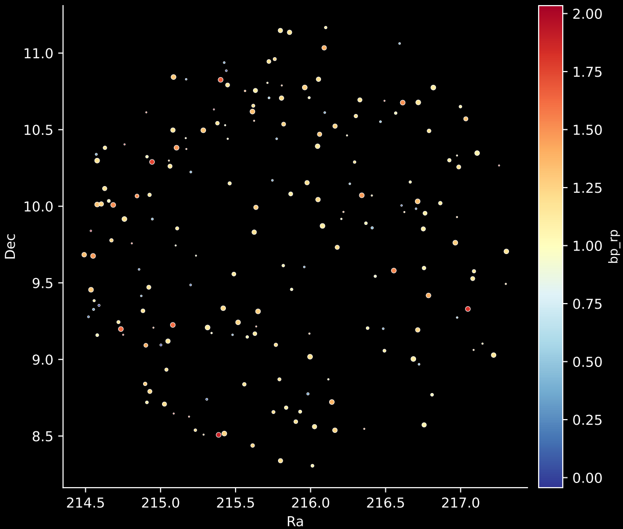
APOGEE DR17 Field: [210+16] Stars: 194
