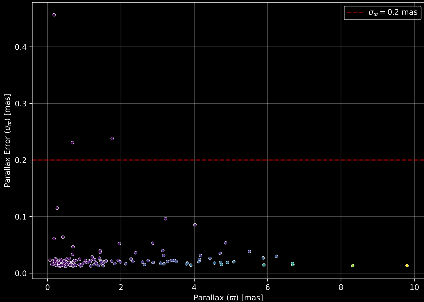
APOGEE DR17 Field: [210+16] Parallax Quality (n= 194)
