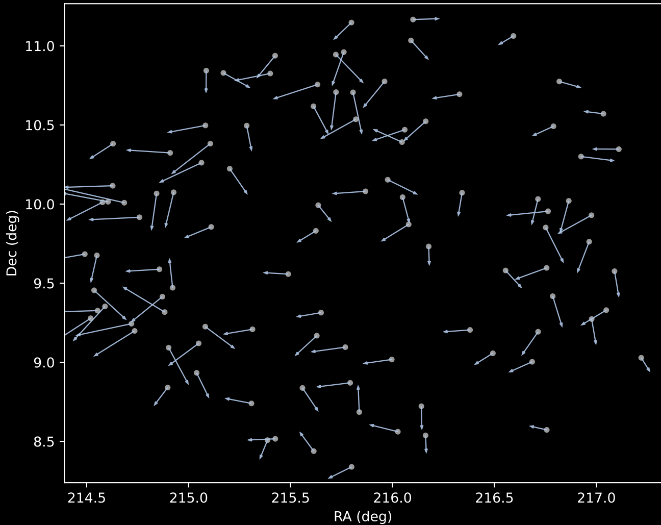
APOGEE DR17 Cluster 1 Proper Motion Vectors (n=100)
