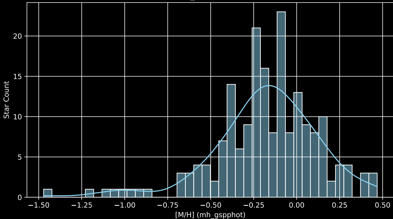
APOGEE DR17 Field: [210+16 [M/H] (mh_gspphot) (n= 192)
