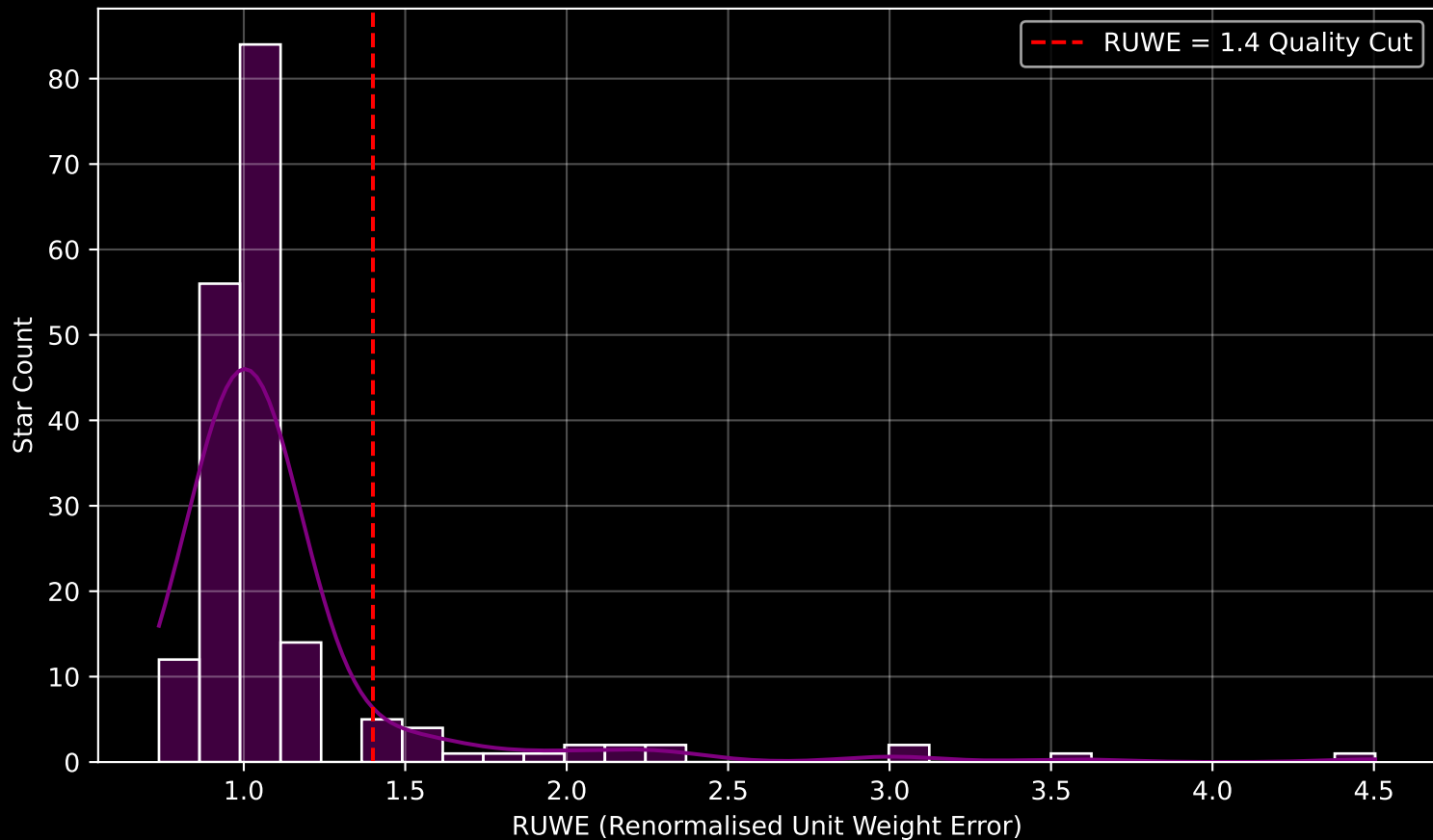
GAPOGEE DR17 Field [210+16] RUWE Distribution (n= 188)
